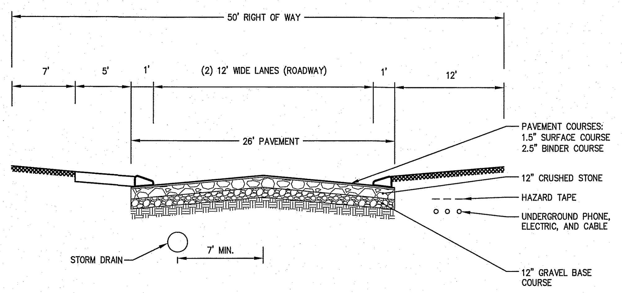
TYPICAL ROAD CROSS SECTION (NOT TO SCALE)
