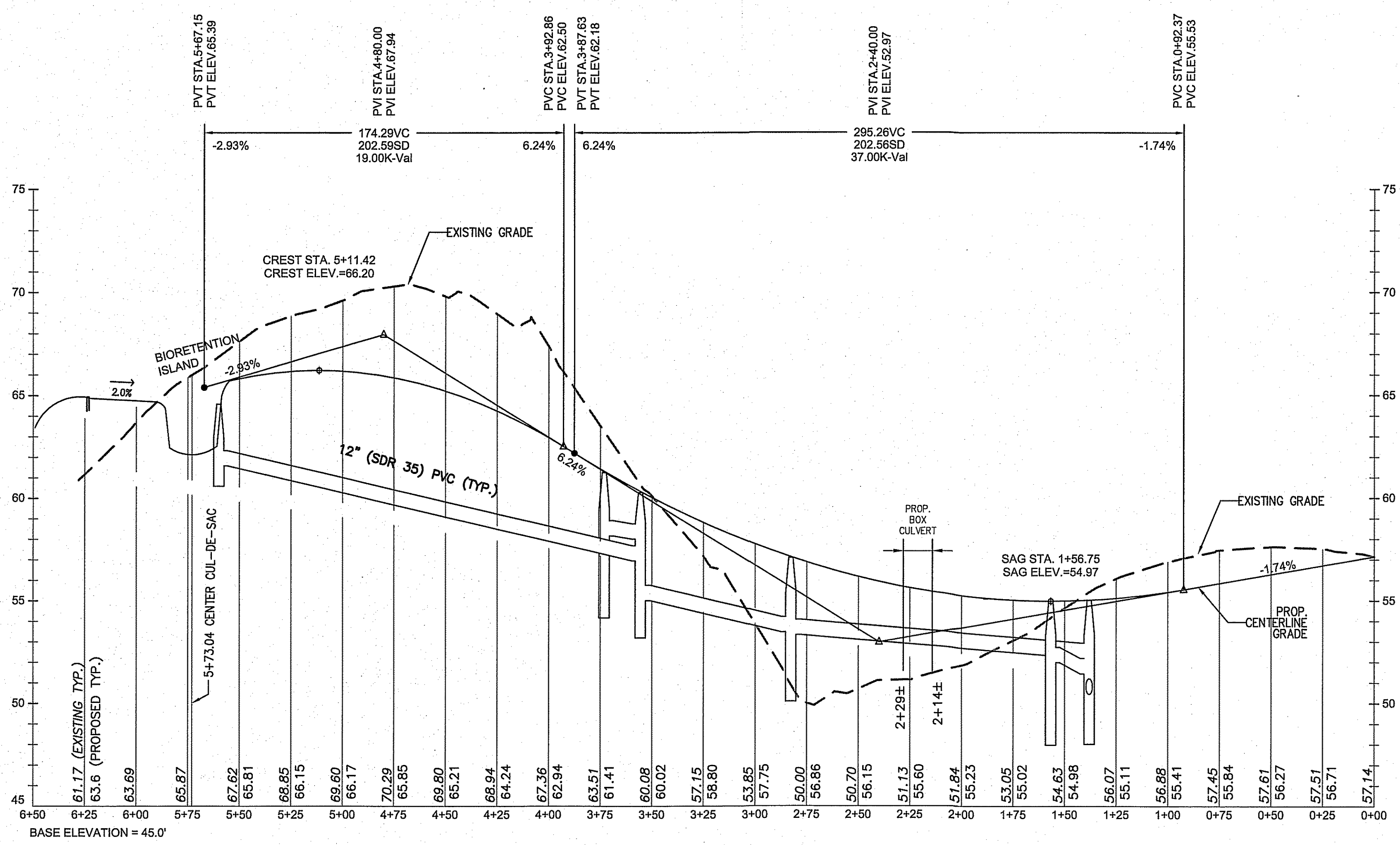
PROPOSED ROAD PROFILE SCALE: 1"=40' (HOR) 1"=4' (VERT)
