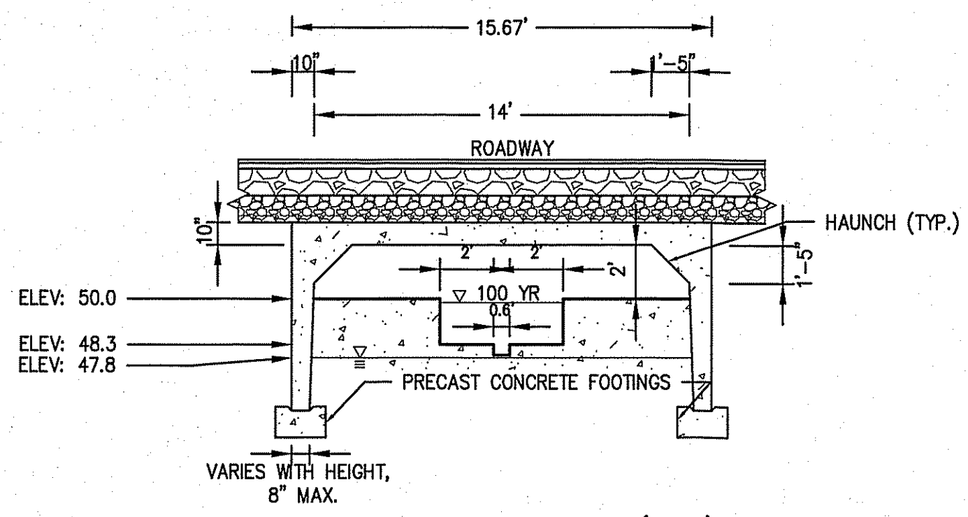
CULVERT CROSS SECTION (B-B) SCALE: 1"=2' (HORIZONTAL & VERTICAL)
